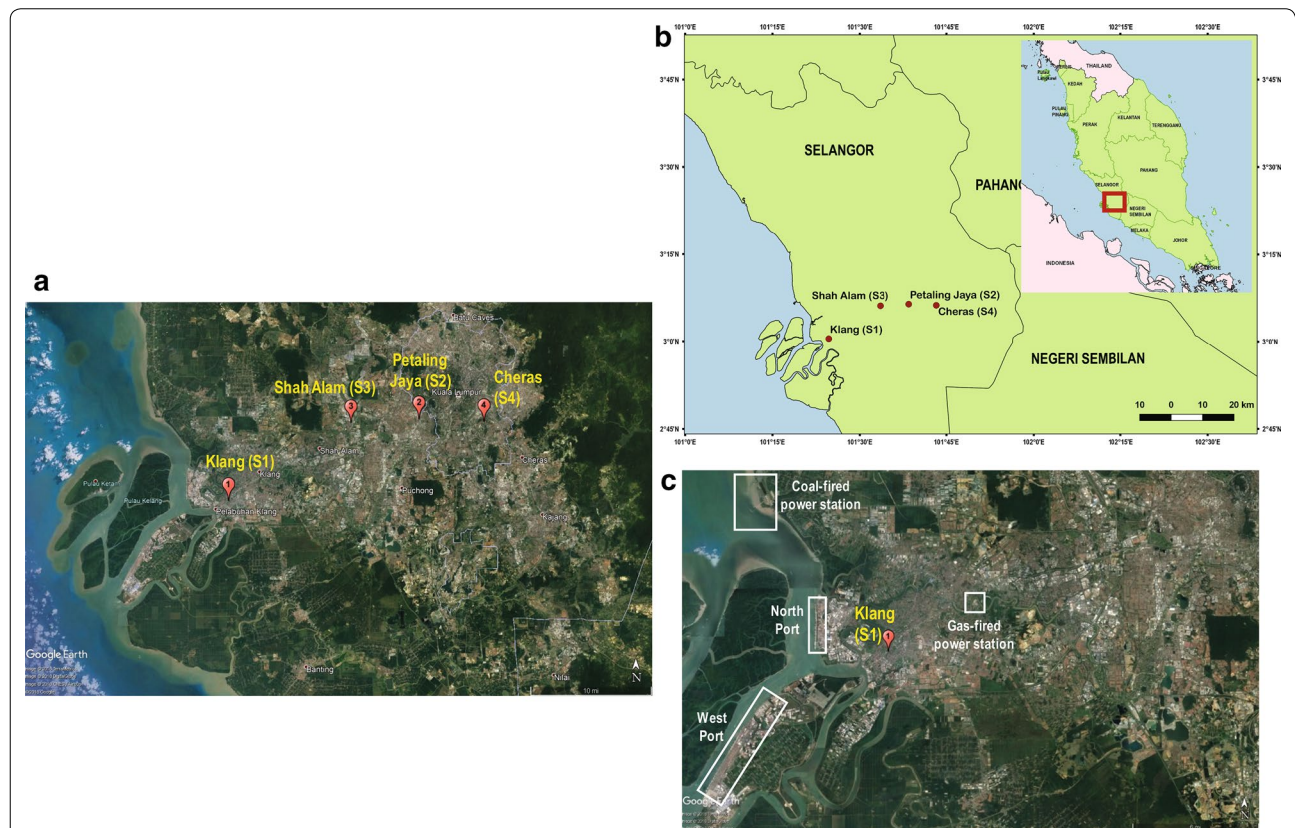
Fig. 1 a Station location of four selected continuous air monitoring stations in urban environment b Location of selected station situated in Peninsular Malaysia c The white boxes in the figure indicate industrial areas surrounding Klang Station
